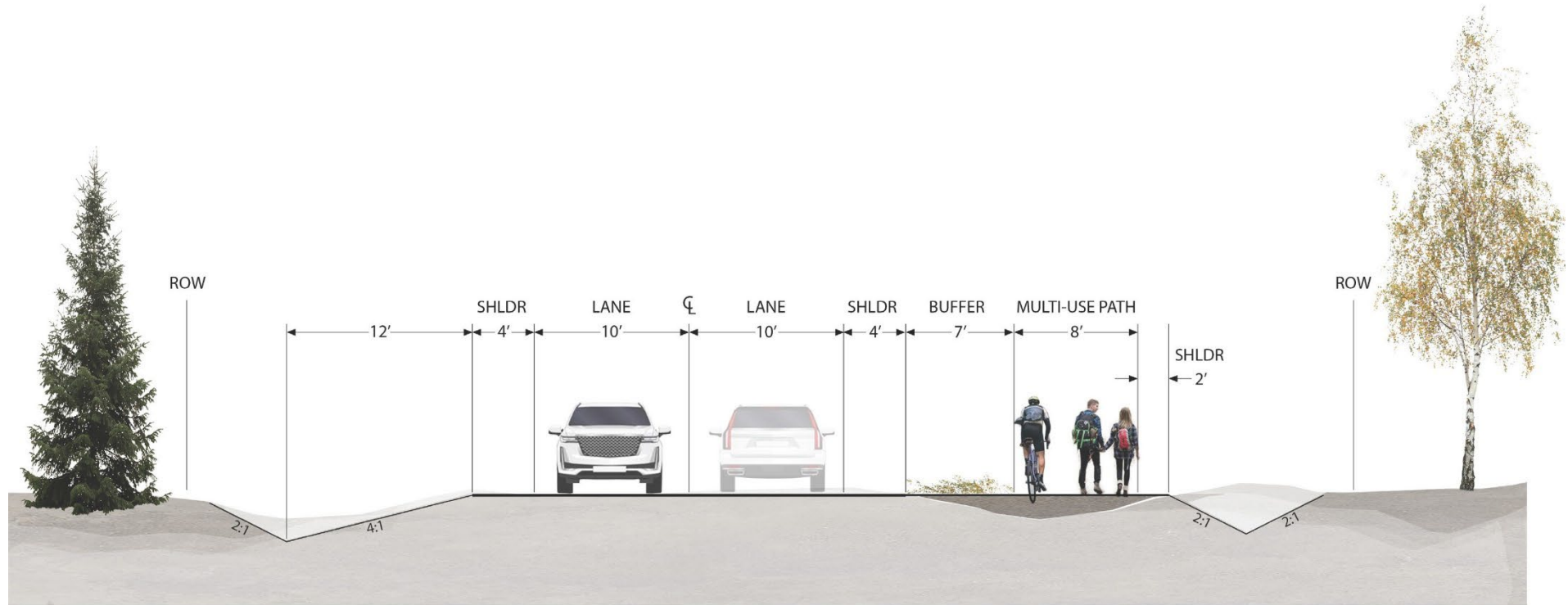
MOUNTAIN AIR DRIVE PRELIMINARY TYPICAL SECTION
